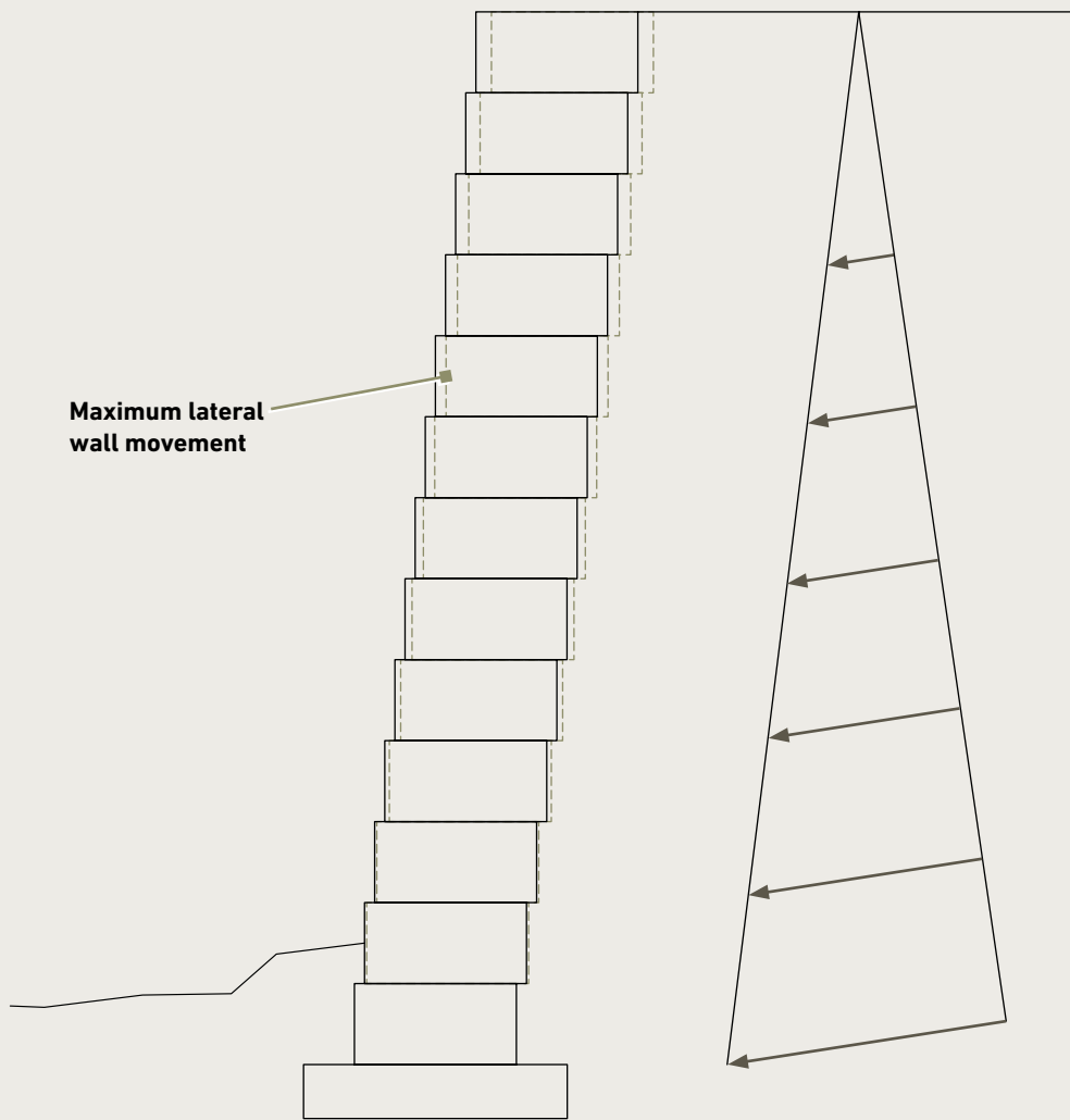
Figure 14.4 | Wall Section
